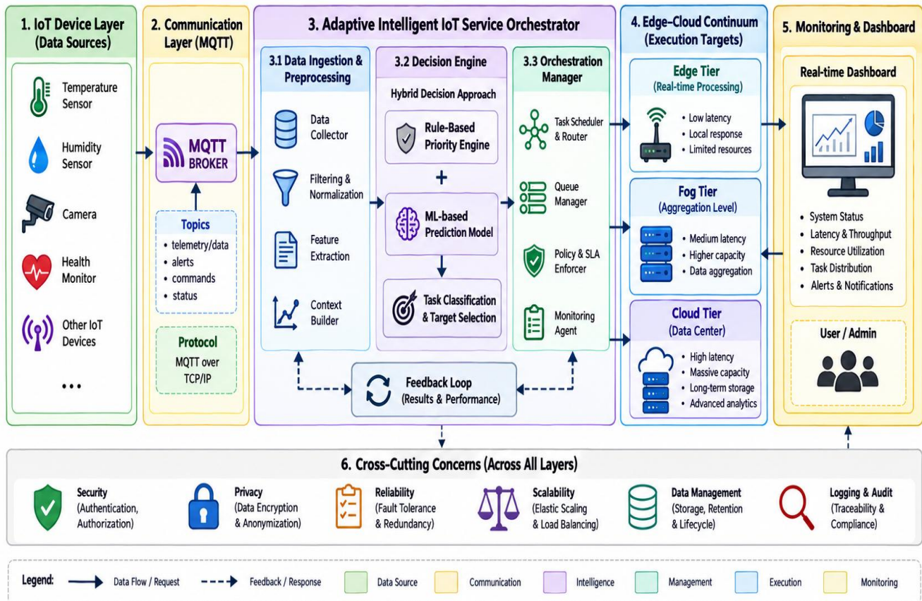
Figure. 2. Task-centric reference architecture for the proposed Adaptive Intelligent IoT Service Orchestrator.
